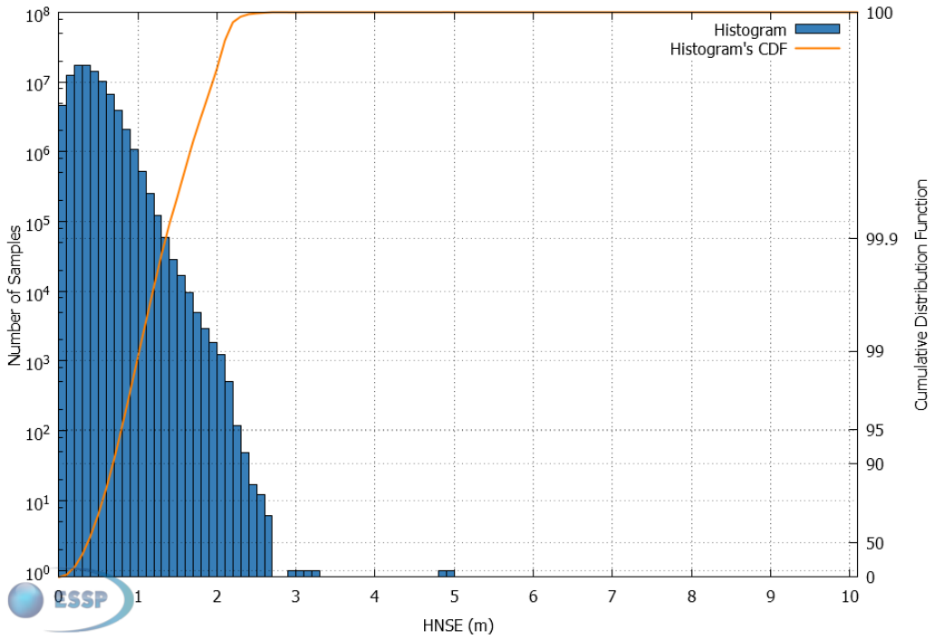
Figure 25 – EGNOS LPV-200 HNSE Histogram and Cumulative Probability
