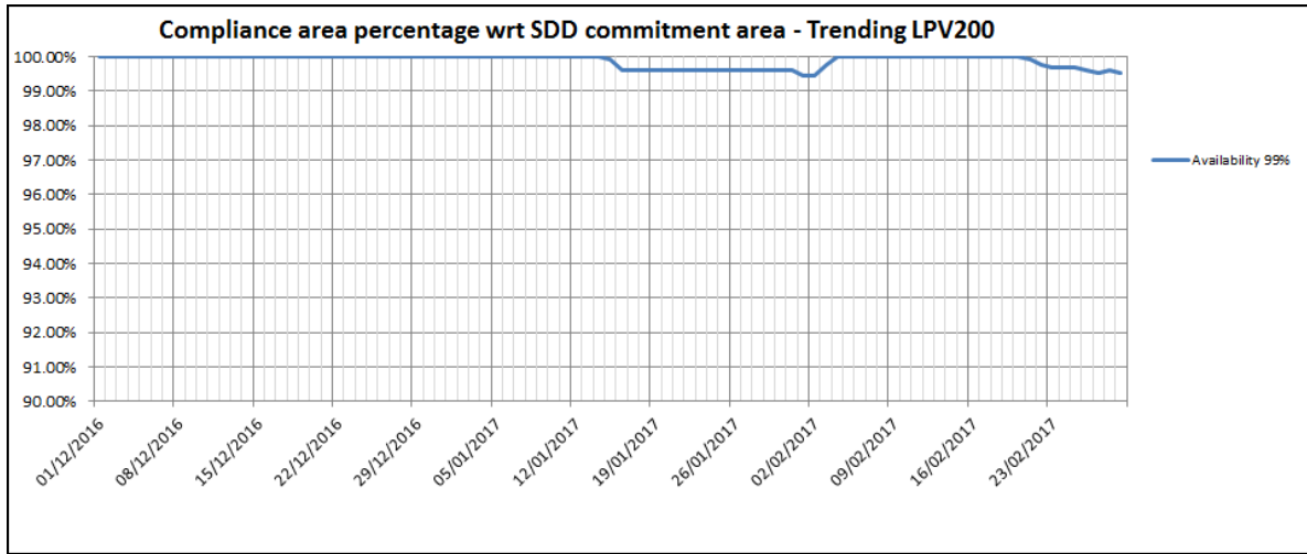
Figure 21 – EGNOS LPV-200 availability compliance trend
