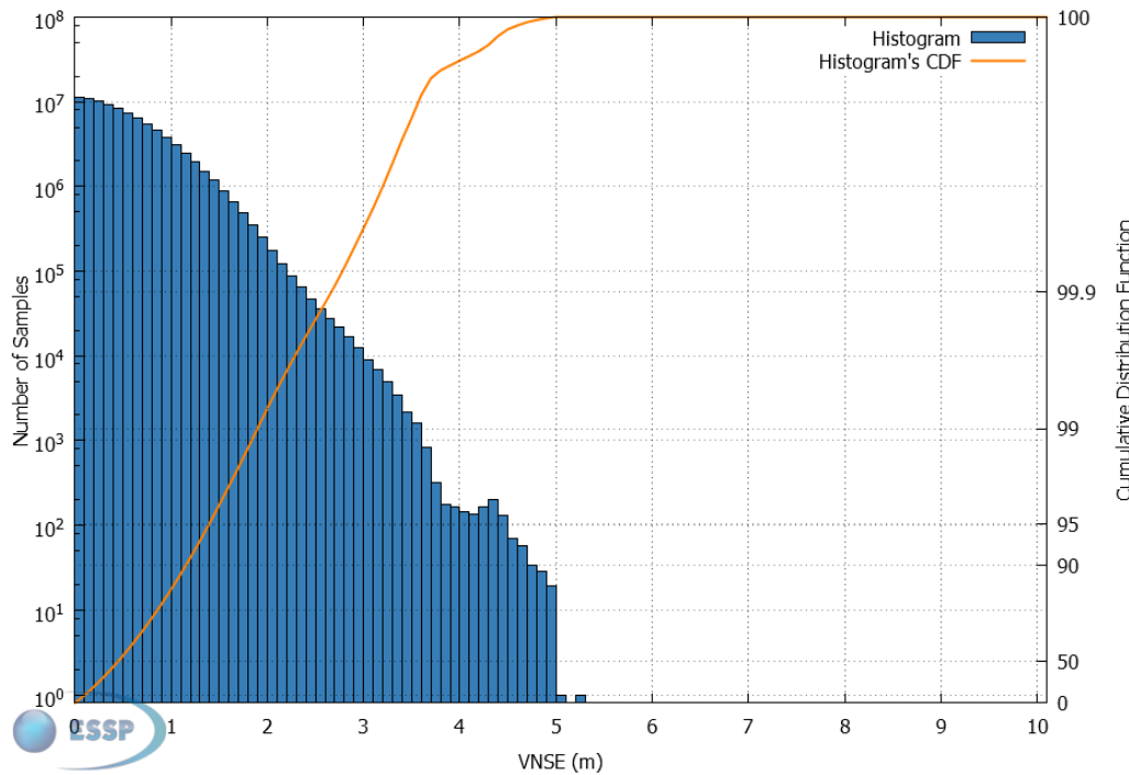
Figure 26 – EGNOS LPV-200 VNSE Histogram and Cumulative Probability
