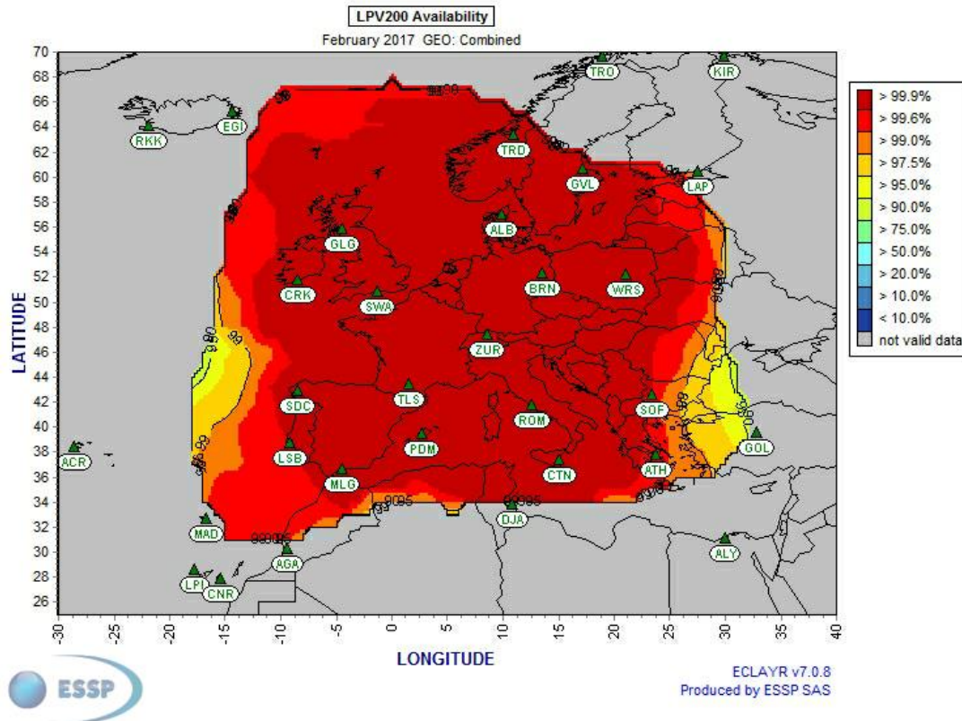
Figure 20 – EGNOS LPV-200 Availability 2
