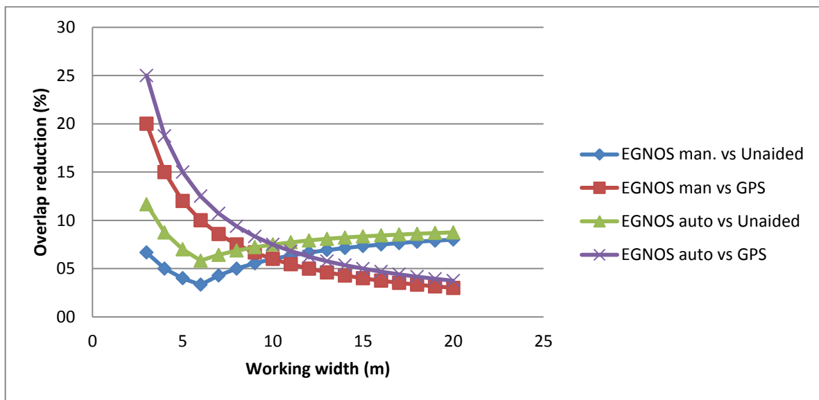
Figure 1: Overlap reduction achieved with EGNOS as a function of the working width.
